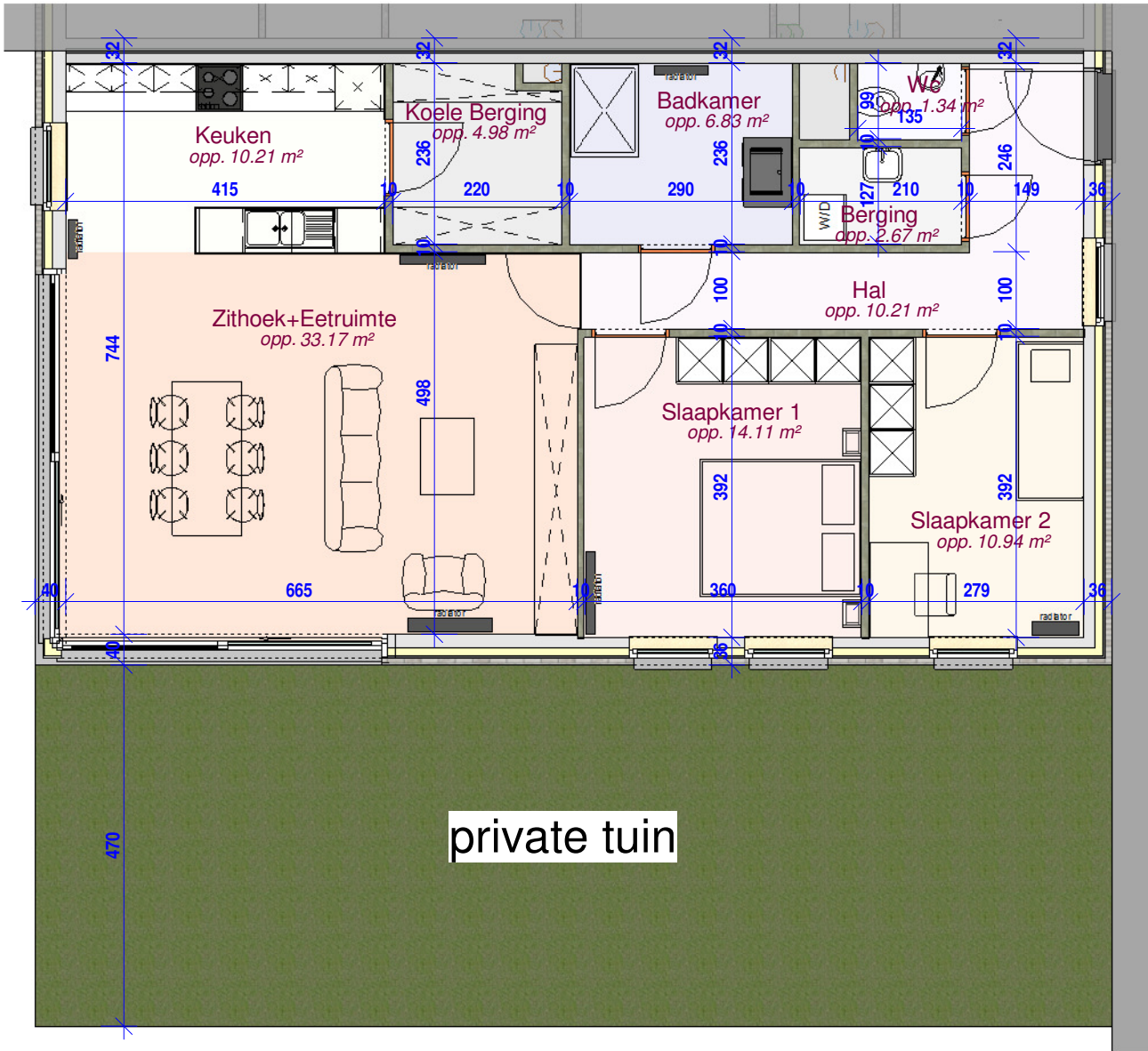
plan A01
