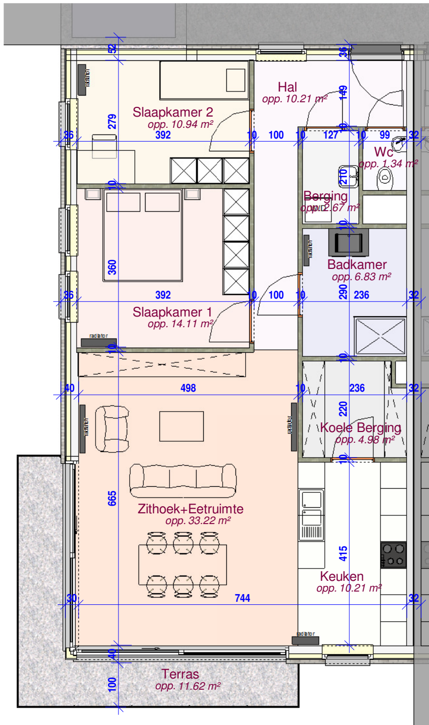
plan A22
