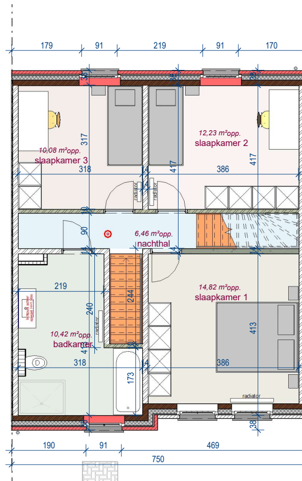
verdieping lot 10
