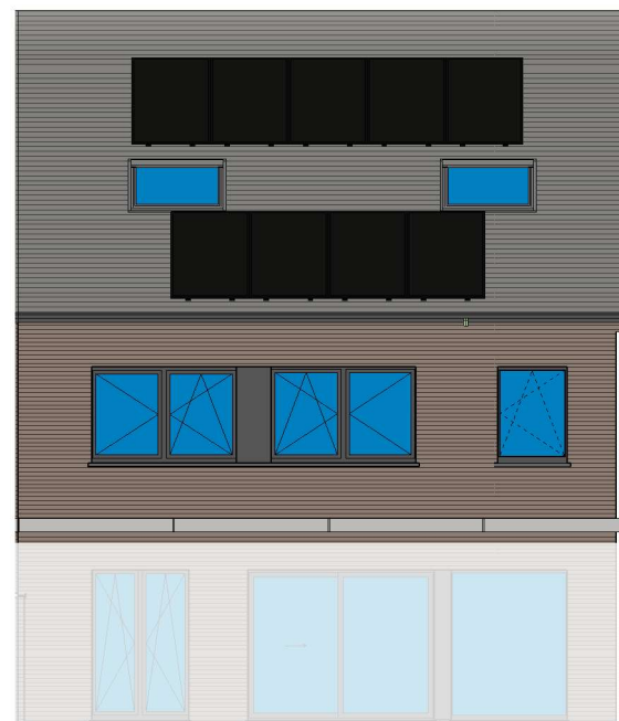
achtergevel lot 15b LL
