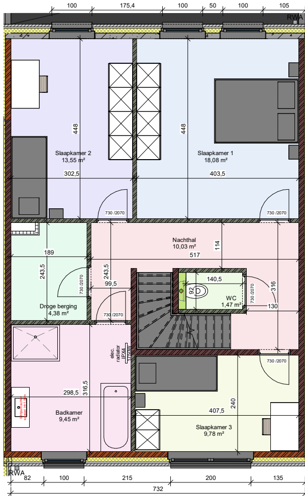
Verdieping LL - lot 2
