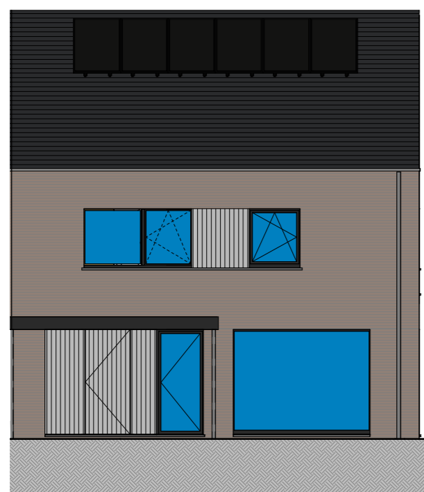
Façade principale lot 40
