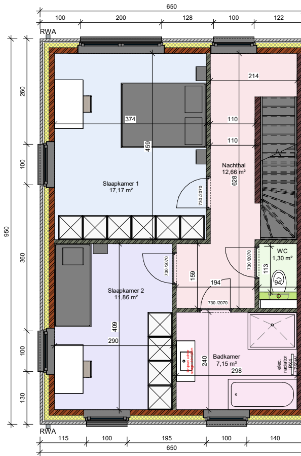
Verdieping LL - lot 7
