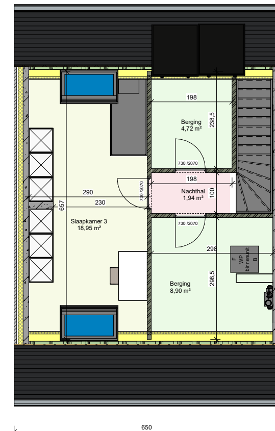
Zolder LL - lot 7
