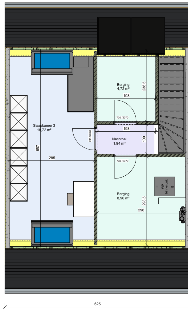
Zolder LL - lot 9
