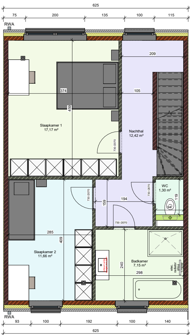
Verdieping LL - lot 9
