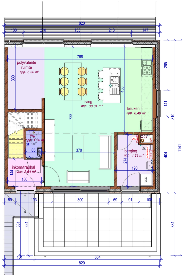
Verdieping lot 9b LL
