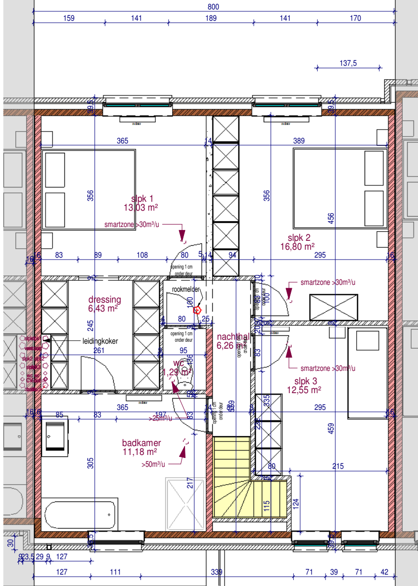
verdieping lot 107
