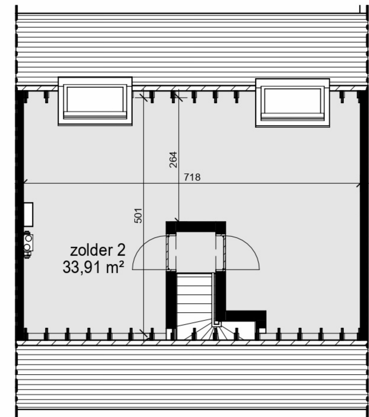
Zolder lot 123 1:75
